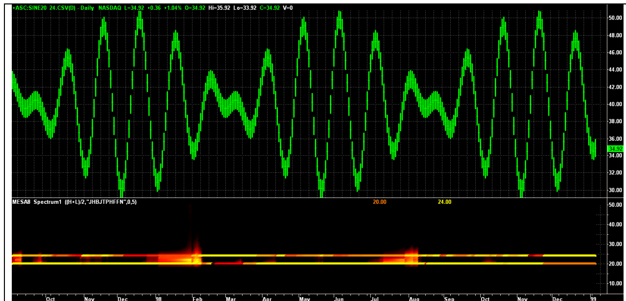
Figure 7. MESA8 Measurement of 20 & 24 Bar Cycles Has High Resolution, Clearly Identifying the Presence of both Components.
